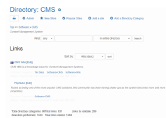
Directory screenshot
